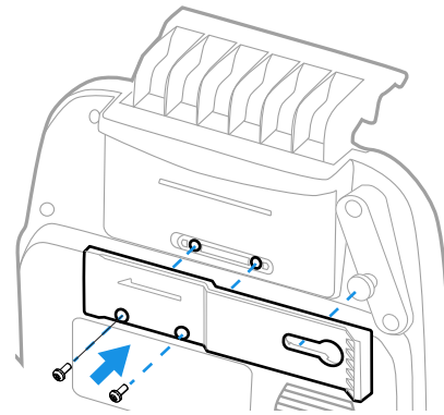
M2.5 x 5 round head screws
